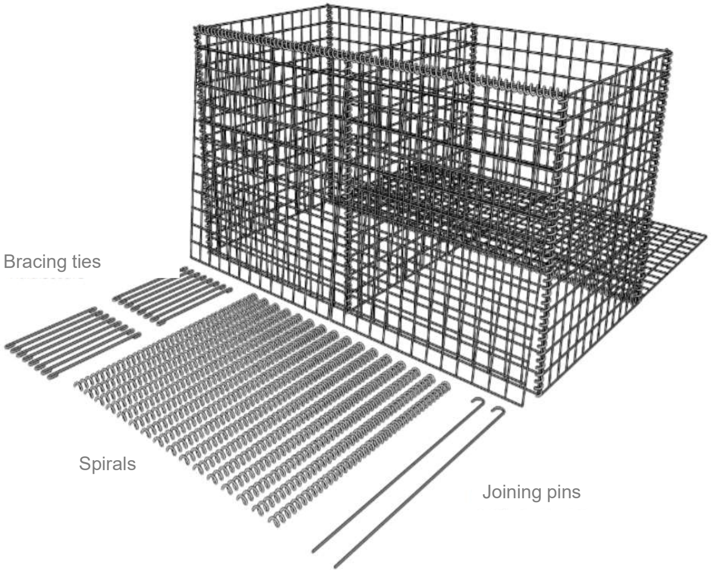
Pre-assembled box
